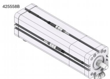
425558B SET saw blade feed cylinder ø50x200mm SET Sägeblattvorschubzylinder ø50x220mm ADN-50*220-S-B
