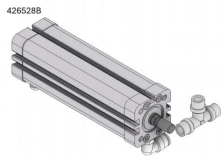
426528B SET cylinder ø32x125 stroke SET Zylinder ø32x125 Hub ADN-32*125-S-B
