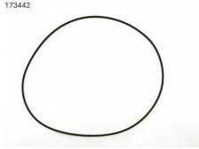
173442 O-ring ø250 x 3,0 mm O-Ring ø250x3,0 NBR 70 Shore
