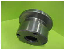
161588 PCE adapter 105-WK \varnothing 105x60mm Adapter PT.PCE \varnothing 105x 60 Winkelkopf
