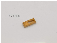
171800 bearing type 3 for roller of short cal. Rollenlager KK RT 4x9x20 Typ3 Carobronze
